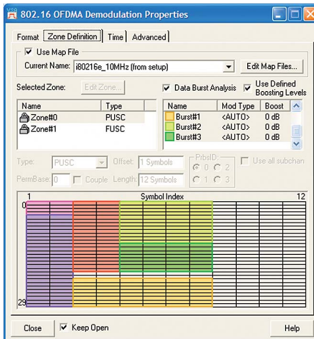
Figure 14. This Zone Definition Grid map was provided by a user map file. The color-coding of the bursts in this map will appear in all the bursts' measurement and error displays.
