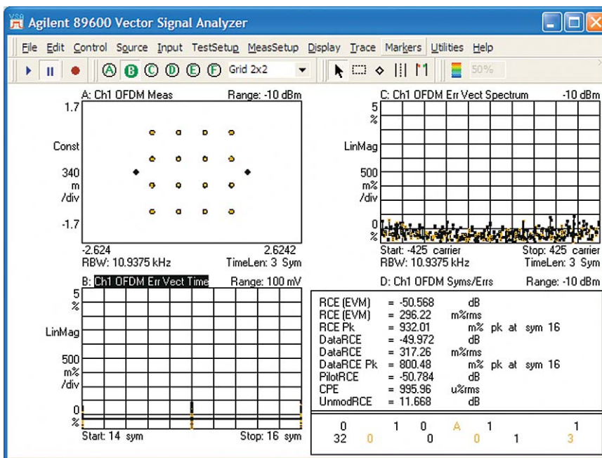
Figure 25. Data burst analysis of a portion of the original burst 2. The error vector time (lower left) trace shows that only 3 symbols are measured, and the error vector spectrum (upper right) shows the sparse OFDM subcarrier population representing the one measured logical subchannel.
