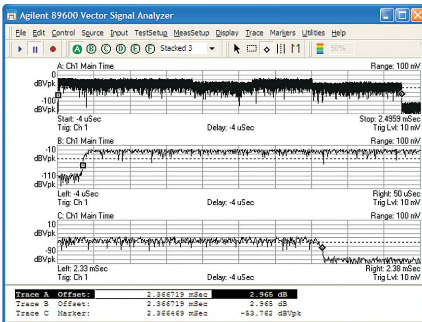
Figure 4. RF envelope of the entire subframe (top trace) along with expanded-scale views of the turn-on and turn-off events (lower traces). Coupled offset markers are used with the expanded scaling to accurately measure the subframe length. Note also the varying power of the RF burst envelope as shown in trace A.
